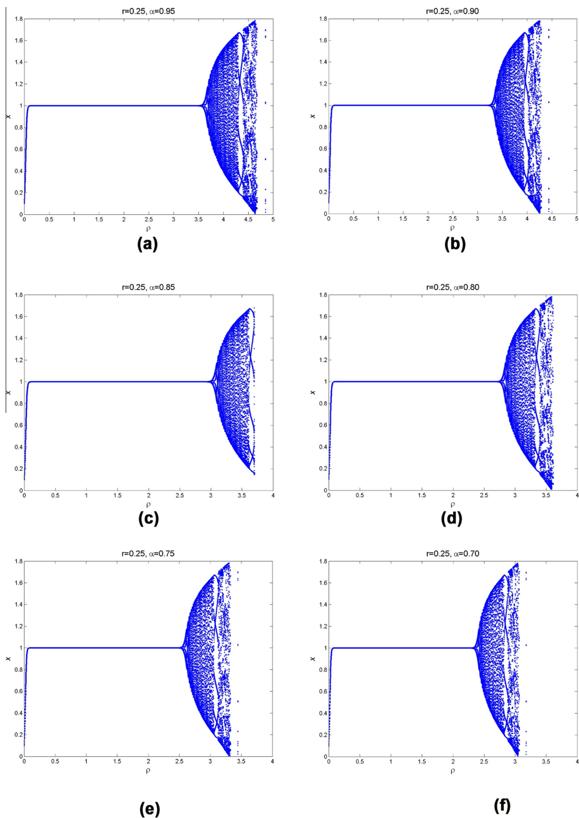
Fig. 2 Bifurcation diagram of system (3.2) as a function of \rho with different values of the fractional-order parameter \alpha .
