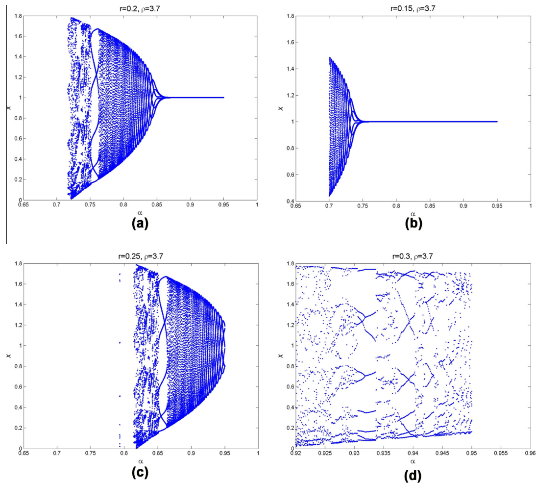
Fig. 3 Bifurcation diagram of system (3.2) as a function of the fractional-order parameter \alpha with different values of the parameters r and \rho .
