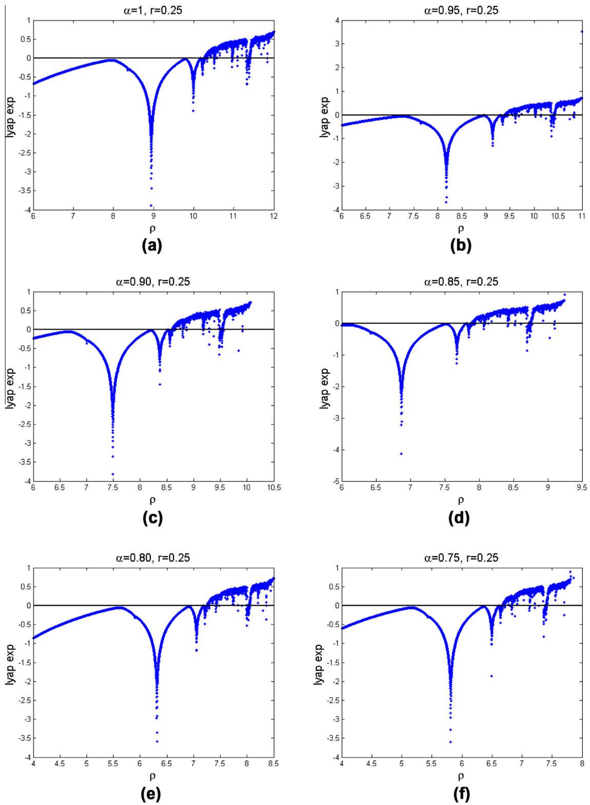
Fig. 1 Lyapunov exponent for system (2.3) with different values of the fractional-order parameter \alpha .
