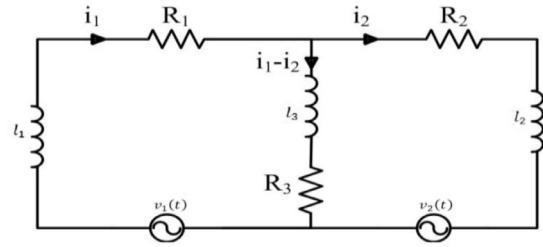
Fig. 1. Electrical circuit of application 1.
